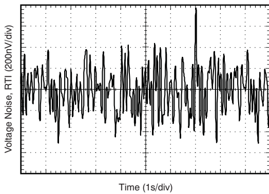
INA282 0.1Hz TO 10Hz VOLTAGE NOISE, RTI
