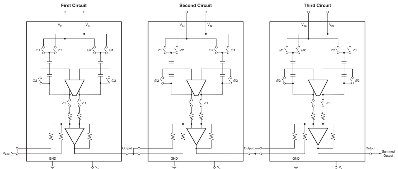
Figure 40. Summing the Outputs of Multiple INA282-Q1 Devices
